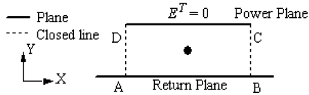
Fig. 5. Sample configuration for calculation of the Poynting vector.
