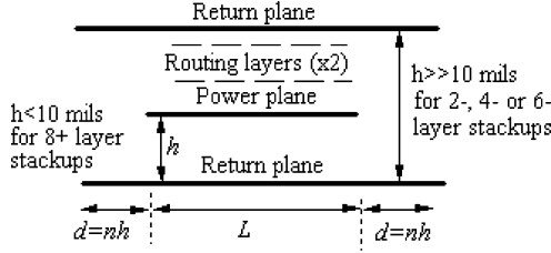
Fig. 2. Planar structure model for all simulation configurations.
