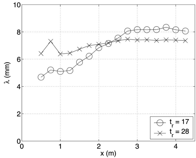
FIG. 42. Taylor microscale \lambda as a function of x (in meters). Space-filling fractal square grids, T=0.91 m tunnel, U_\infty=12 m/s. For the t_r=17 grid, x_{peak} \approx 2.75 m and for the t_r=28 grid, x_{peak} \approx 3.2 m. In both cases, \lambda is approximately constant where x > x_{peak} .
