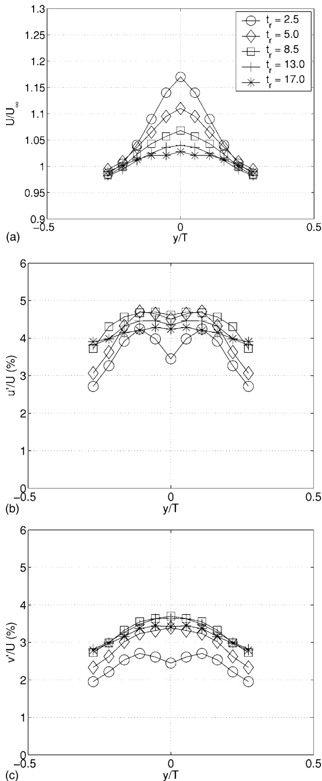
FIG. 35. Homogeneity mean profiles, space-filling square grids, T = 0.46 m tunnel, U_\infty=10 m/s, x=3.25 m.
