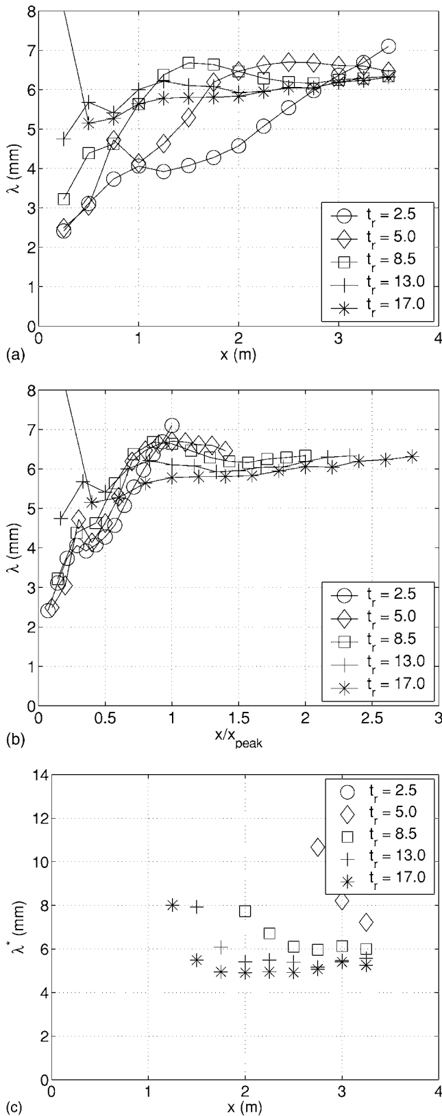
FIG. 41. Taylor microscales \lambda and \lambda^* as functions of x (in meters) and x/x_{peak} . Space-filling fractal square grids, T=0.46 m tunnel, U_\infty=10 m/s.
