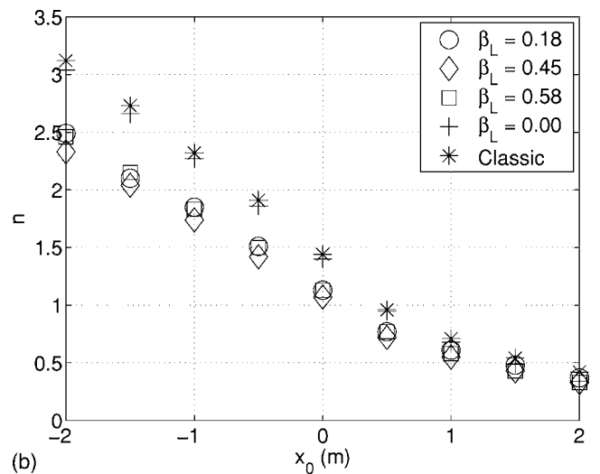
FIG. 10. Exponents s and n as functions of x_0 , T=0.91 m tunnel, U_\infty=12 m/s. See Fig. 3 for grid correspondence with \beta_L .
