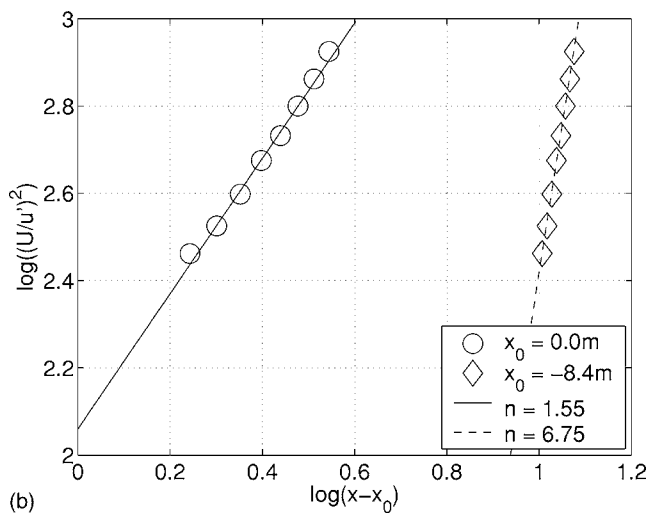
FIG. 43. Taylor microscale \lambda (in millimeters) as a function of x-x_0 (in meters) and \log(U/u')^2 as a function of \log(x-x_0) for two values of x_0 with power-law best-fit curves through data. The best-fit values of s and n for each x_0 are given in the plots. Space-filling fractal square grid t_r=17 , T=0.46 m tunnel, U_\infty=10 m/s.
