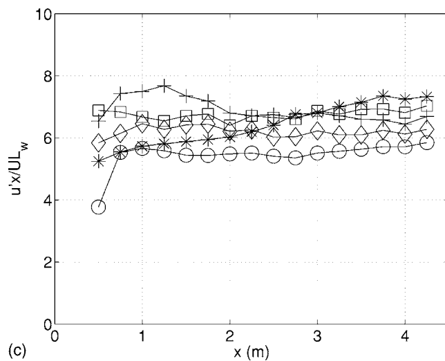
FIG. 30. Permanence of large eddies, I grids in T=0.91 m tunnel, U_\infty=12 m/s.
