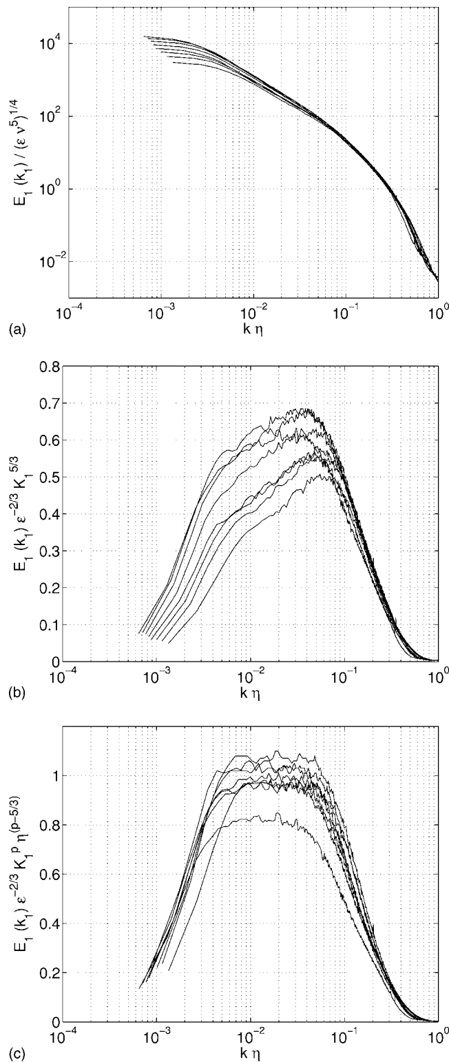
FIG. 47. Energy spectra at x=3.25 m downstream the t_r=13 fractal square grid in the T=0.46 m tunnel at eight different speeds U_z ranging between 6 and 20 m/s in 2 m/s increments.
