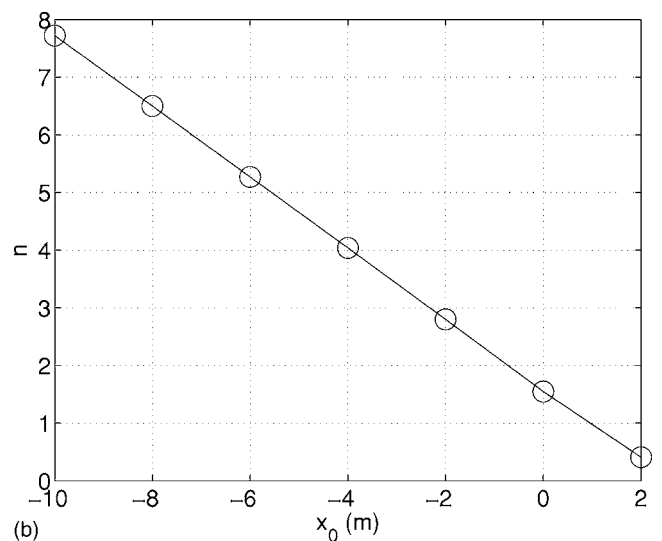
FIG. 44. Exponents s , s^* , and n as functions of x_0 (in meters). Space-filling fractal square grids t_r=17 , T=0.46 m tunnel, U_\infty=10 m/s.
