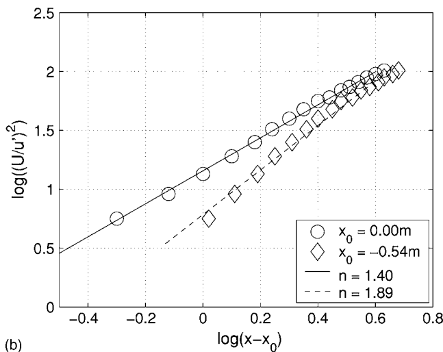
FIG. 9. Cross grid with \sigma=40\% , T=0.91 m tunnel, U_\infty=12 m/s.
