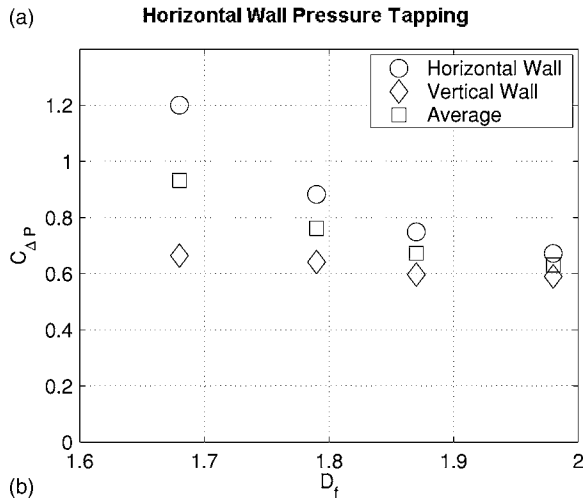
FIG. 14. Pressure tappings and C_{\Delta P} values for different D_f . T=0.91 m tunnel.
