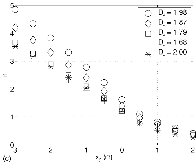
FIG. 29. I grids in T=0.91 m tunnel, U_\infty=12 m/s. Exponents s , s^* , and n as functions of x_0 (in meters).
